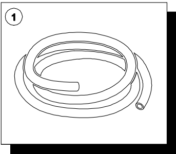
Hose I.D.: 19 mm (3/4") O.D.: 30 m Working pressure: 225 p.s.i. Burst pressure: 675 p.s.i. Weight: 0.580 kg/m
