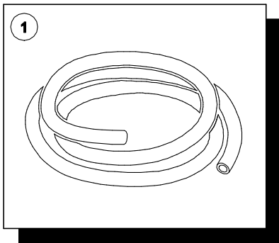
Hose I.D.: 19 mm (3/4") O.D.: 30 mm Working pressure: 15.5 bar (225 psi) Burst pressure: 46.54 bar (675 psi) Weight: 0.580 kg/m
