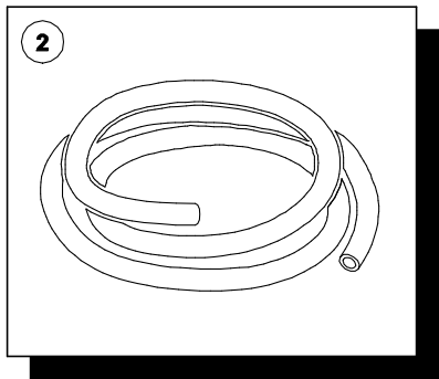
Hose I.D.: 25 mm (1") O.D.: 36 mm Working pressure: 15.5 bar (225 psi) Burst pressure: 46.54 bar (675 psi) Weight: 0.830 kg/m
