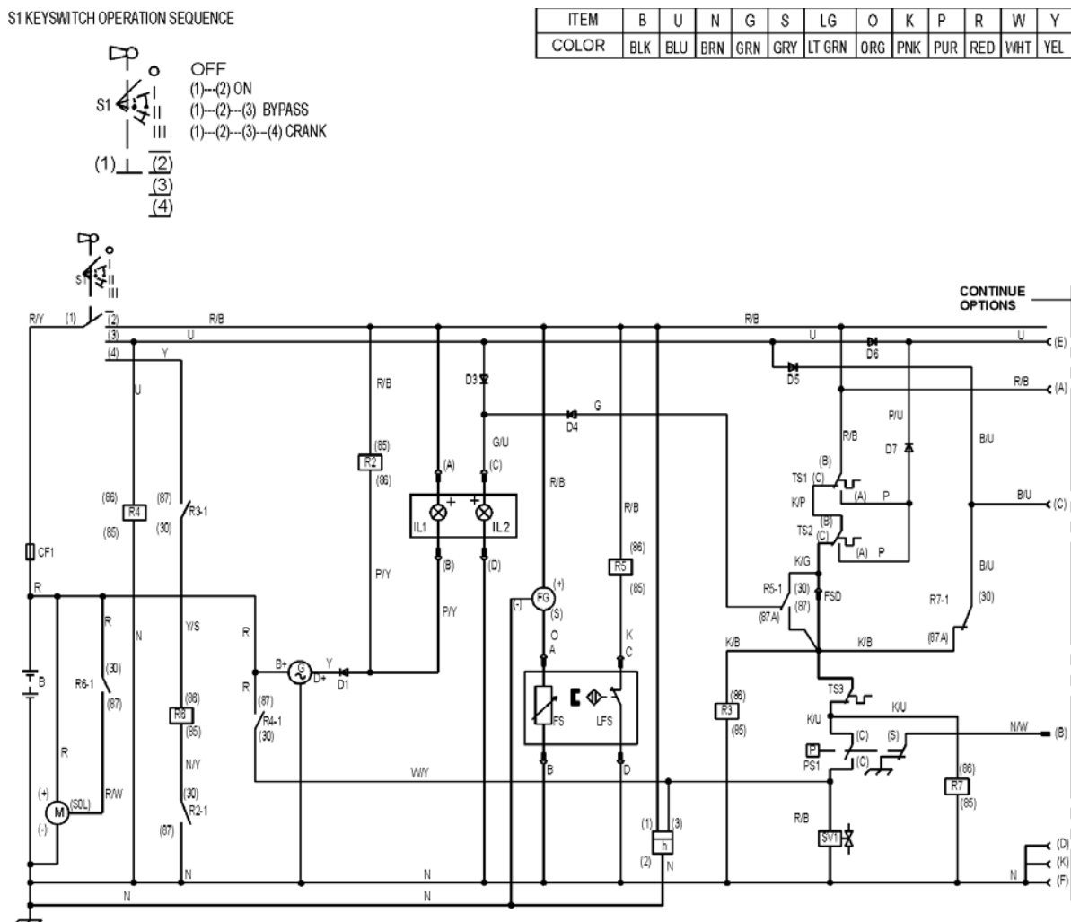
S1 KEYSWITCH OPERATION SEQUENCE
