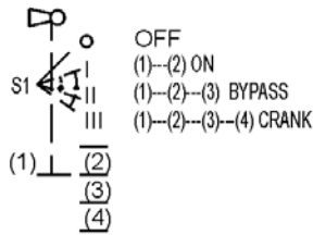
S1 KEYSWITCH OPERATION SEQUENCE
