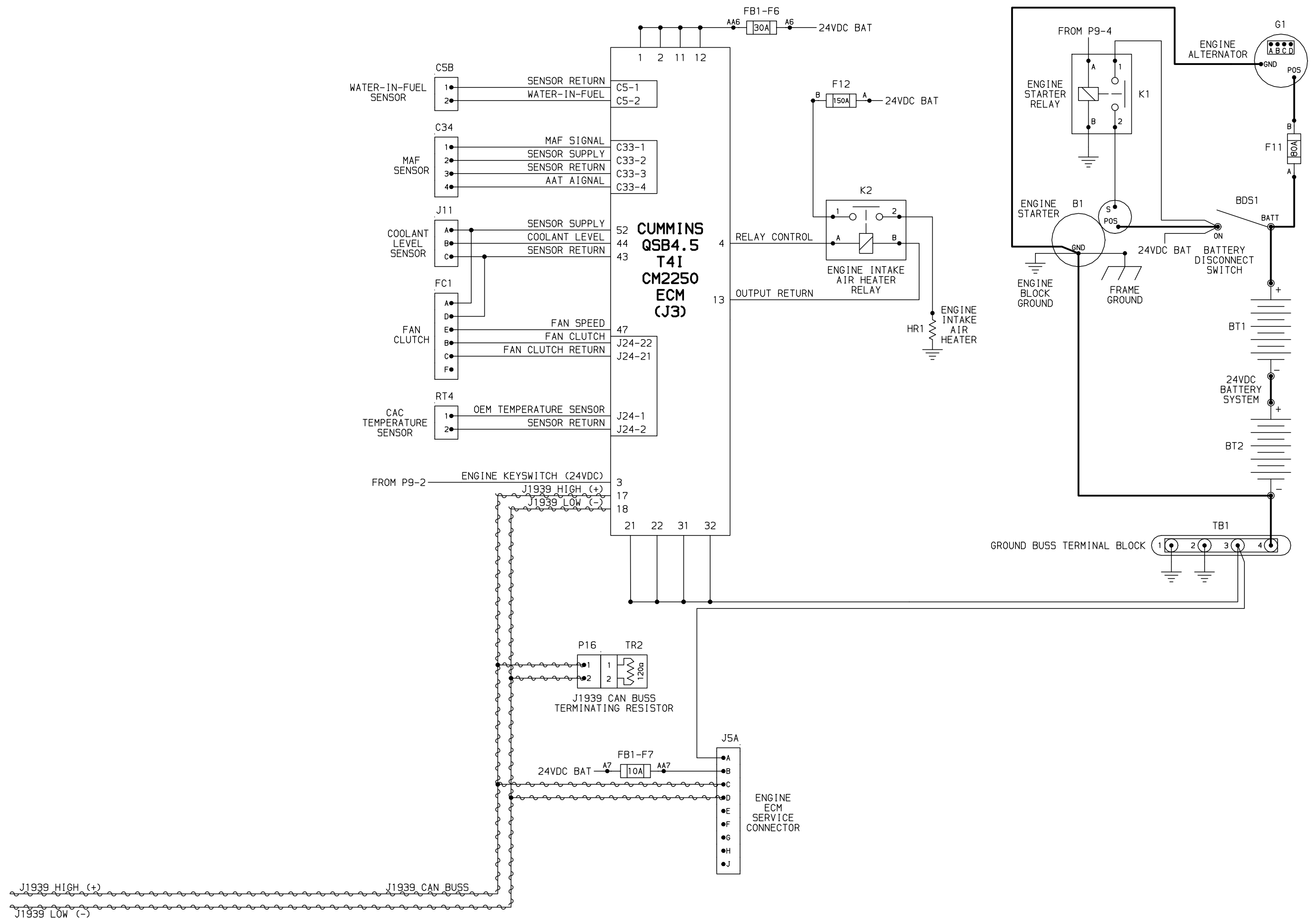
Compressor and Engine Control System Schematic 46582499 Rev.B (sheet 3)
