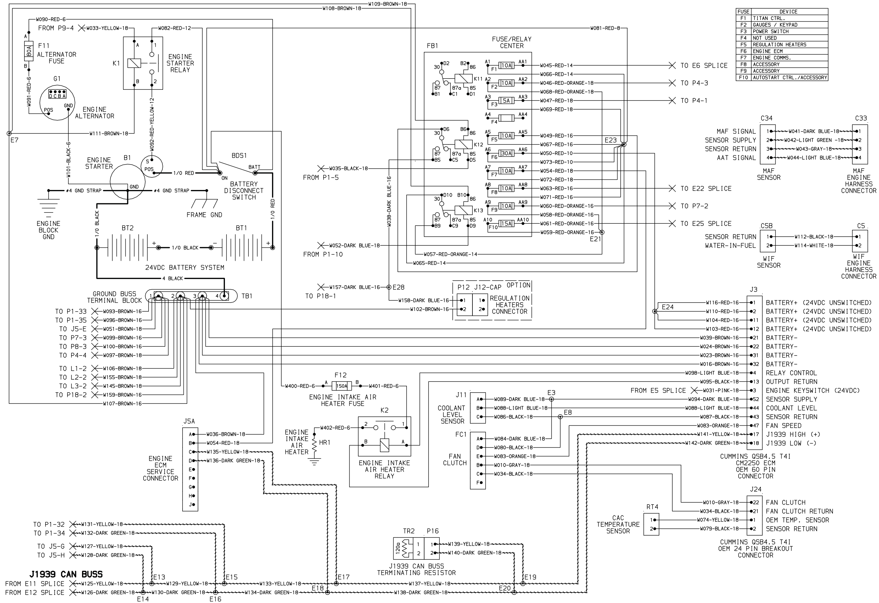
Compressor & Engine Harness Schematic 46582500 Rev.D (sheet 2)
