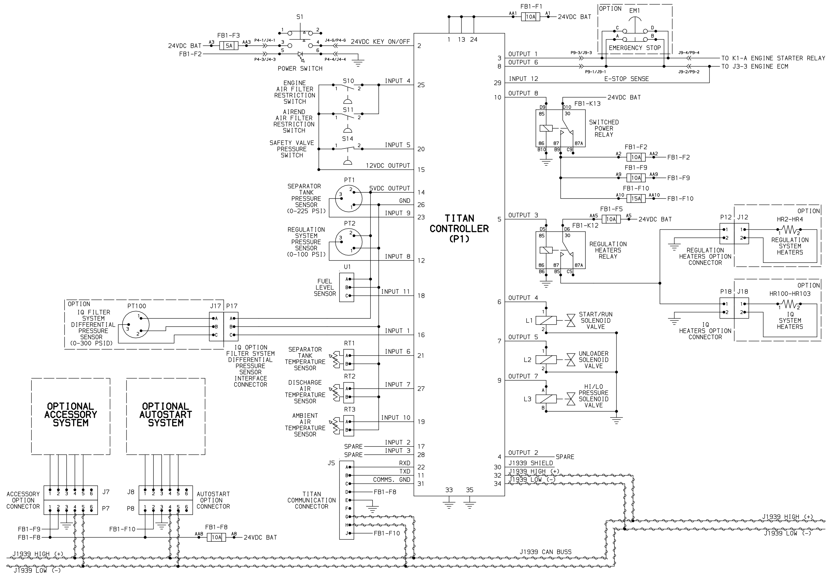
Compressor and Engine Control System Schematic 46582499 Rev.B (sheet 2)
