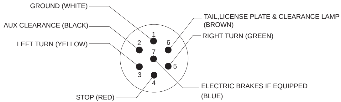
STOP, TAIL & TURN LIGHT OPTION (AS VIEWED FROM REAR OF SOCKET)
