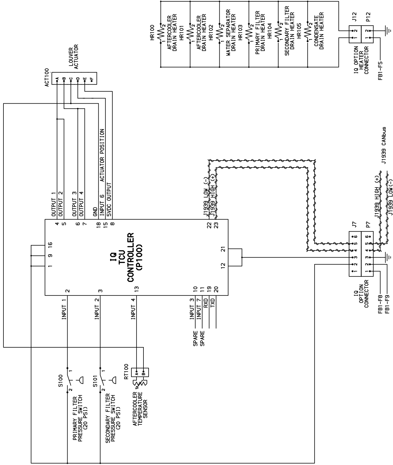
IQ Option Harness Control System Schematic 46670349 Rev. A
