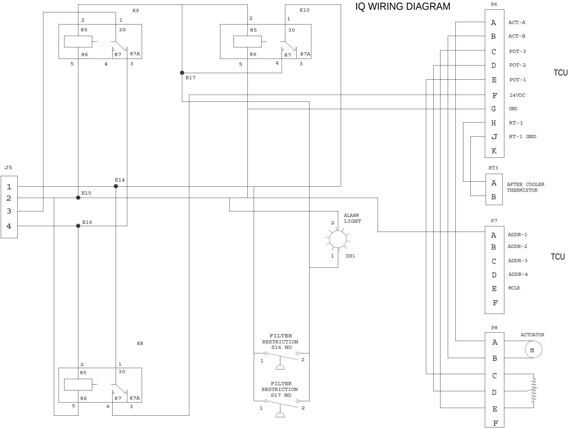
IQ Wiring Diagram
