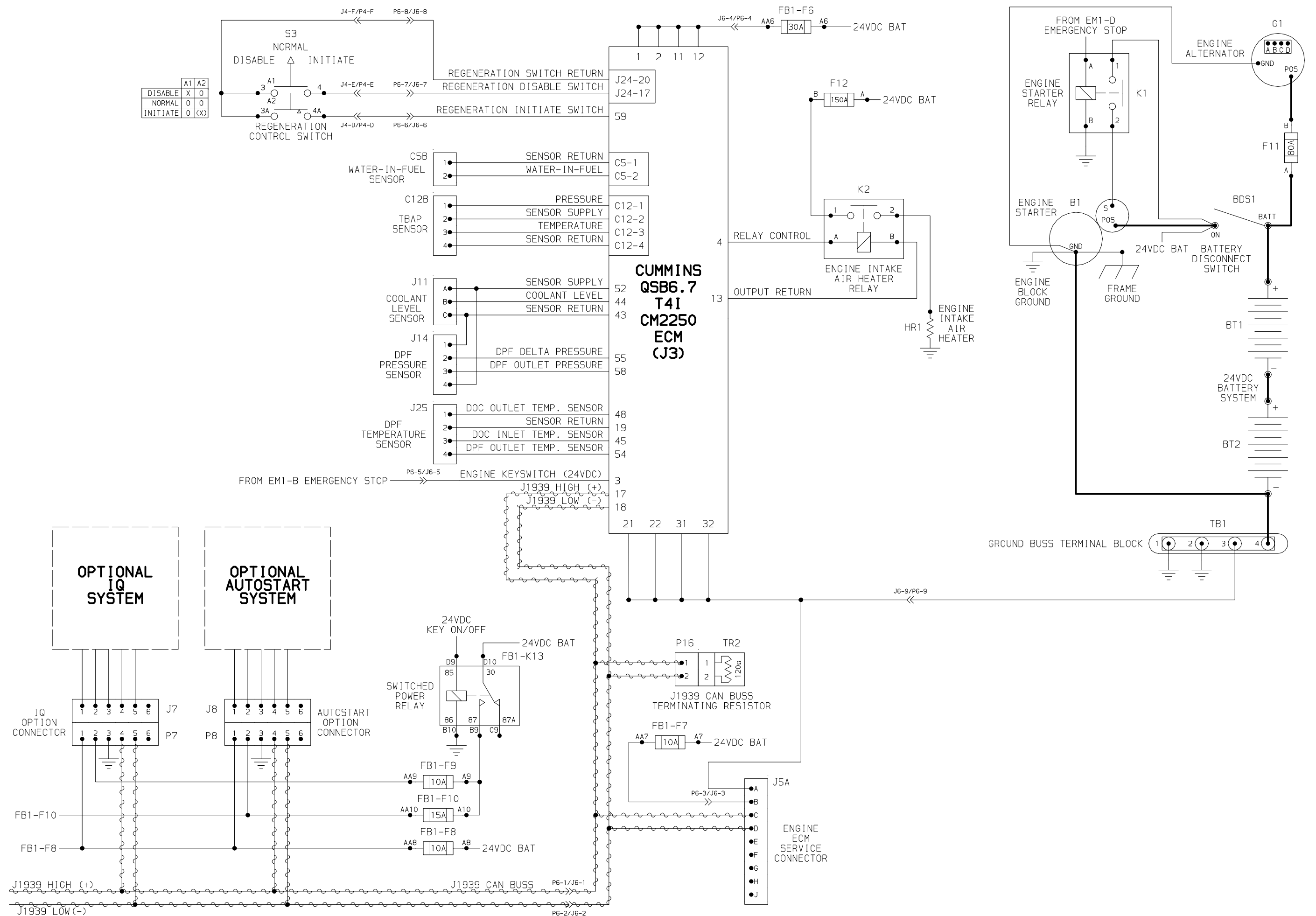
Compressor and Engine Control System Schematic 46559019 Rev.C (sheet 2)
