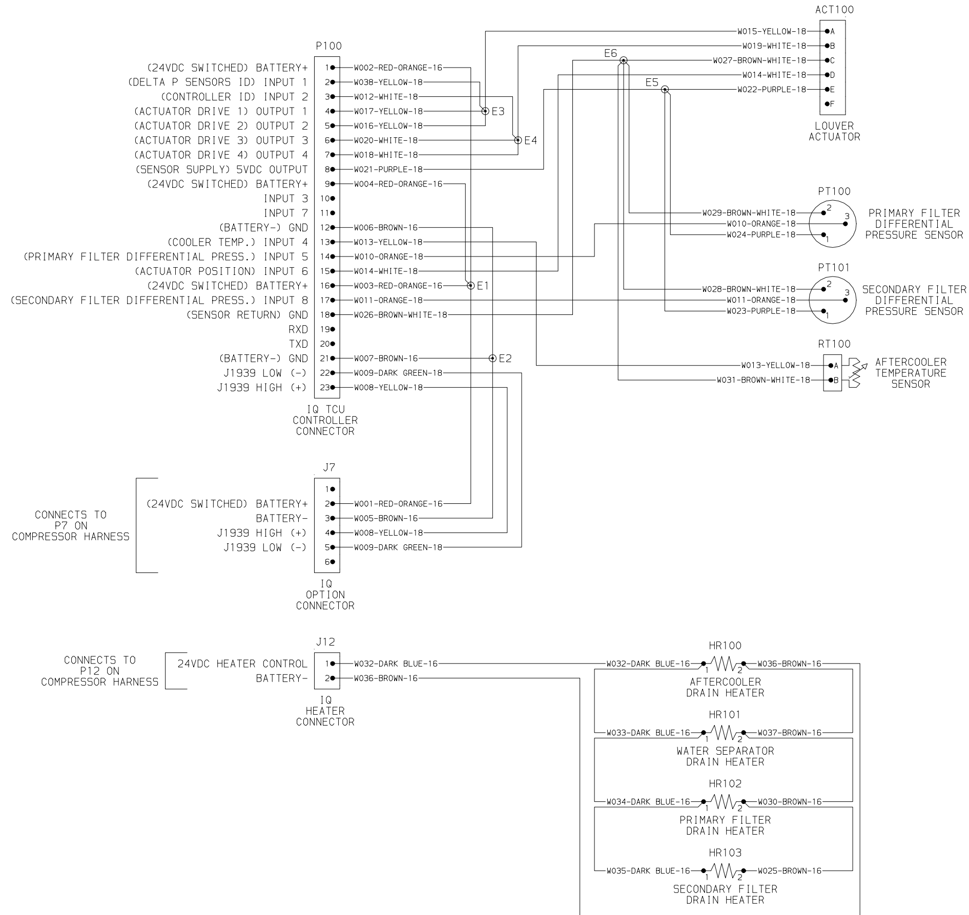
IQ Option Harness Schematic 46599620 Rev.A
