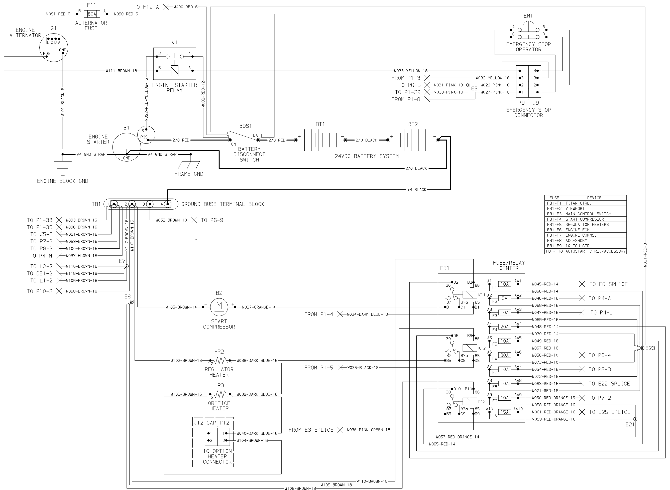
Compressor and Engine Harness Schematic 46559020 Rev.D (sheet 3)
