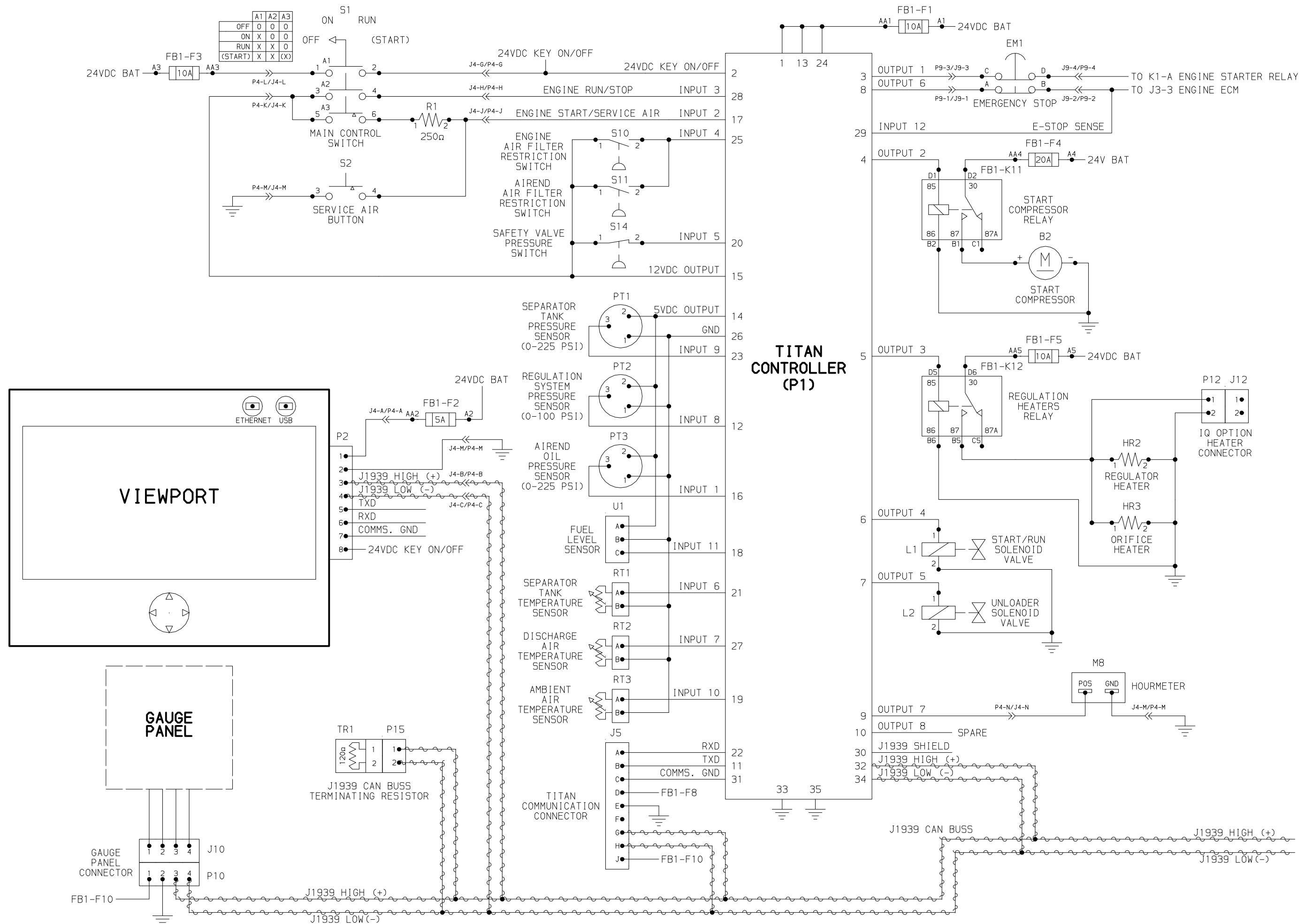
Compressor and Engine Control System Schematic 46559019 Rev.C (sheet 1)
