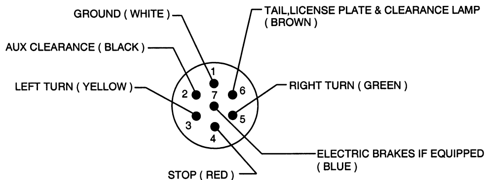
STOP, TAIL & TURN LIGHT OPTION ( AS VIEWED FROM REAR OF SOCKET )
