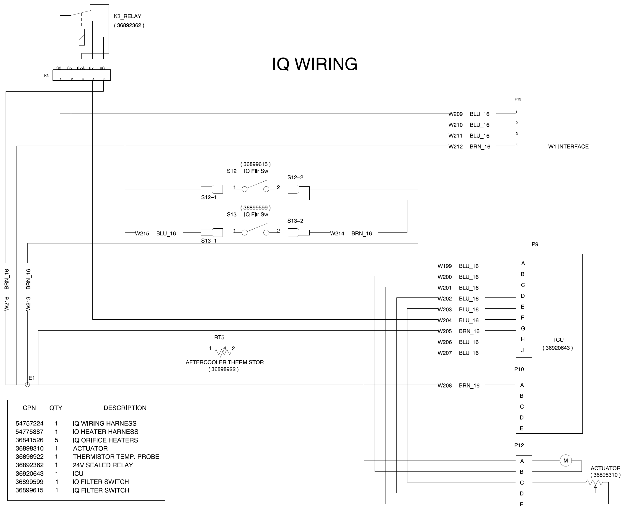
IQ Wiring Diagram
