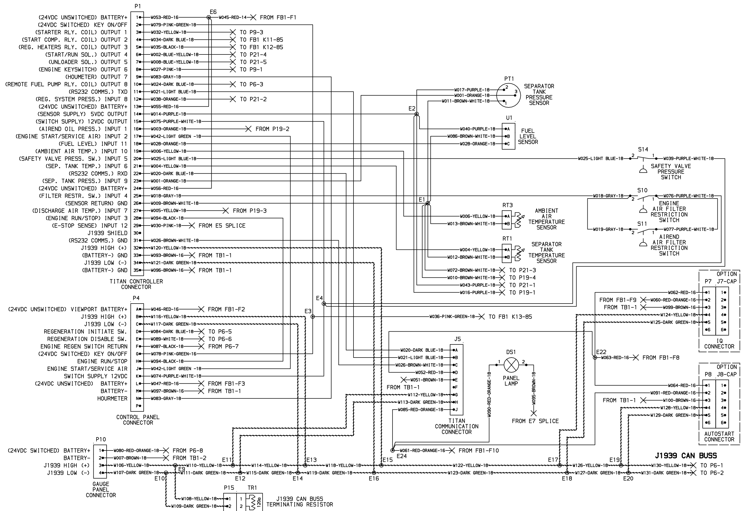
Compressor & Engine Harness Schematic 46609000 Rev.C (sheet 1)
