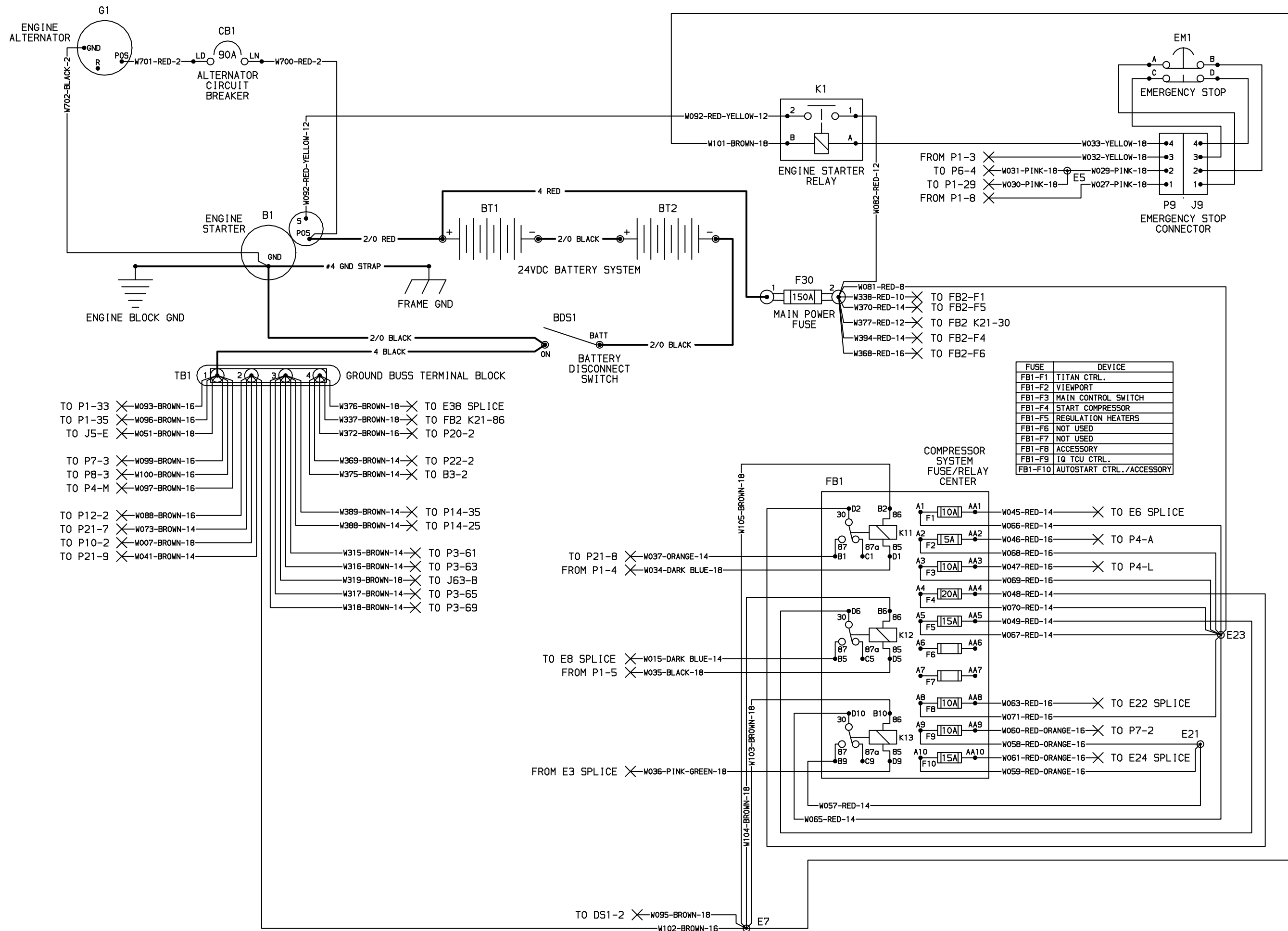
Compressor & Engine Harness Schematic 46609000 Rev.C (sheet 4)
