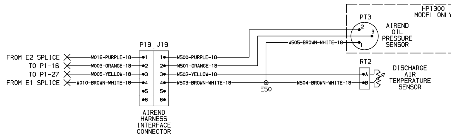
Compressor & Engine Harness Schematic 46609000 Rev.C (sheet 5)
