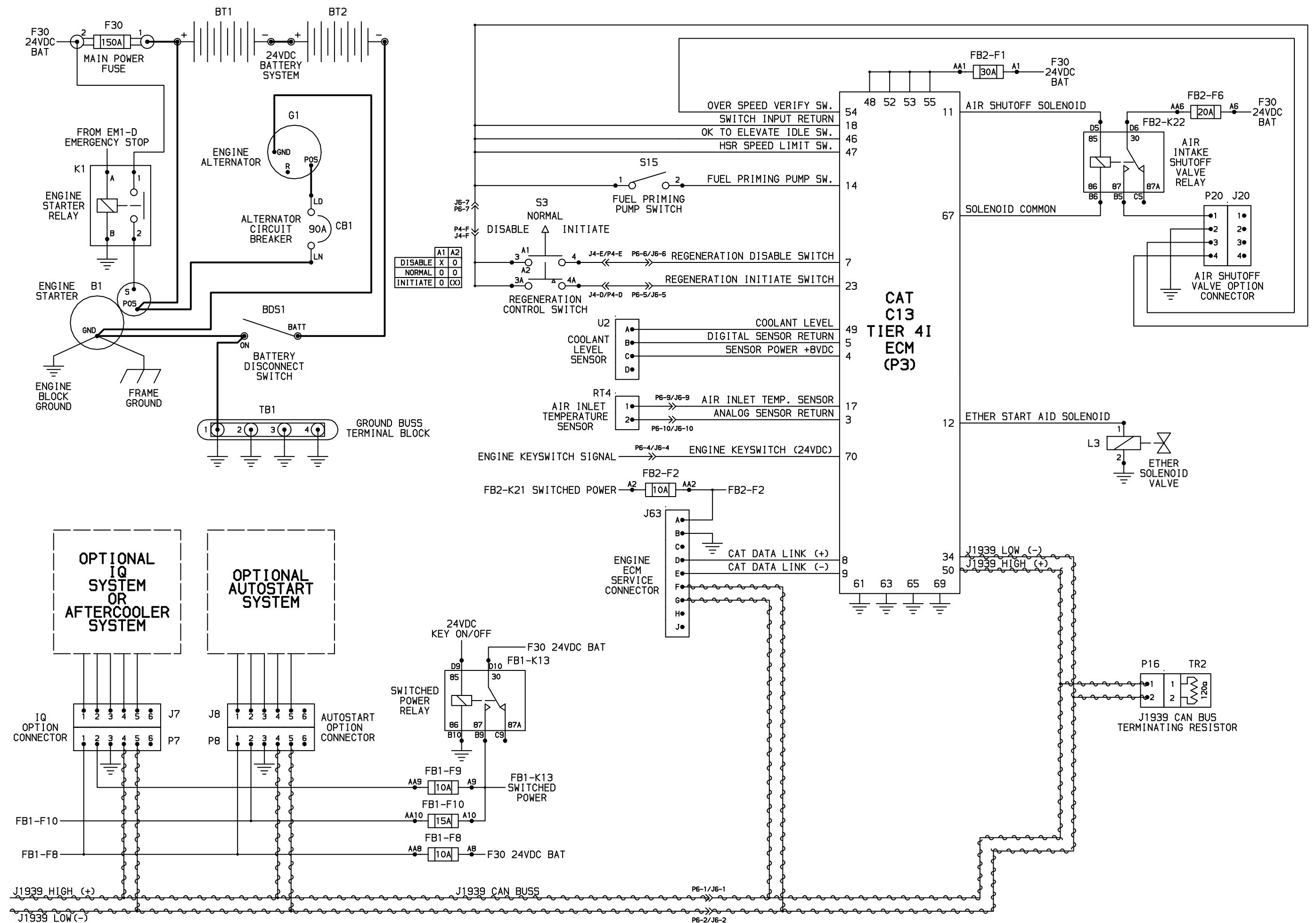
Compressor & Engine Control System Schematic 46608999 Rev.C (sheet 2)
